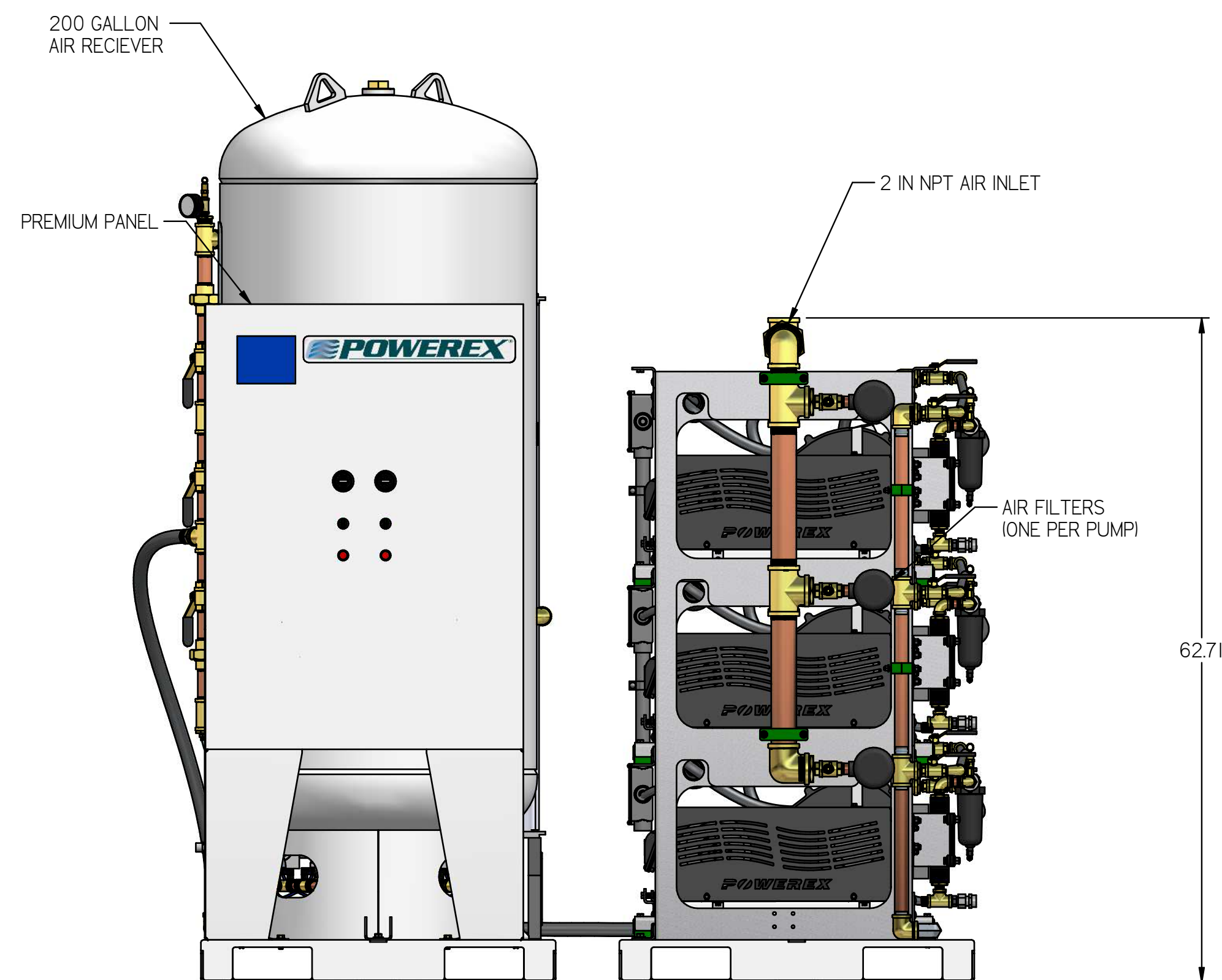
FRONT VIEW
