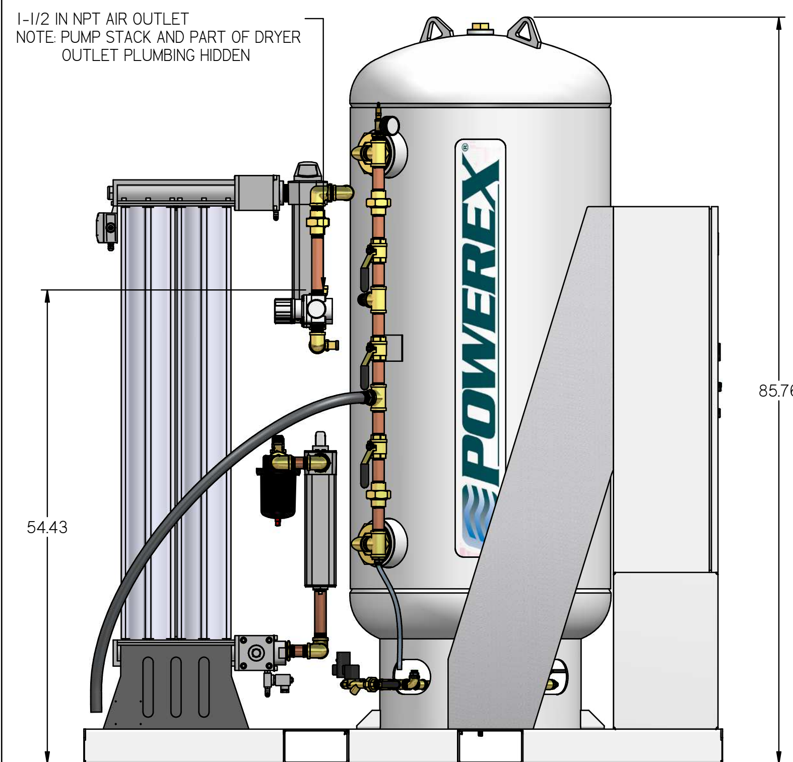
LEFT VIEW
